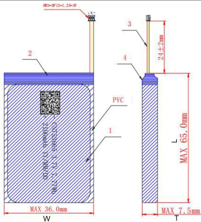
Battery
